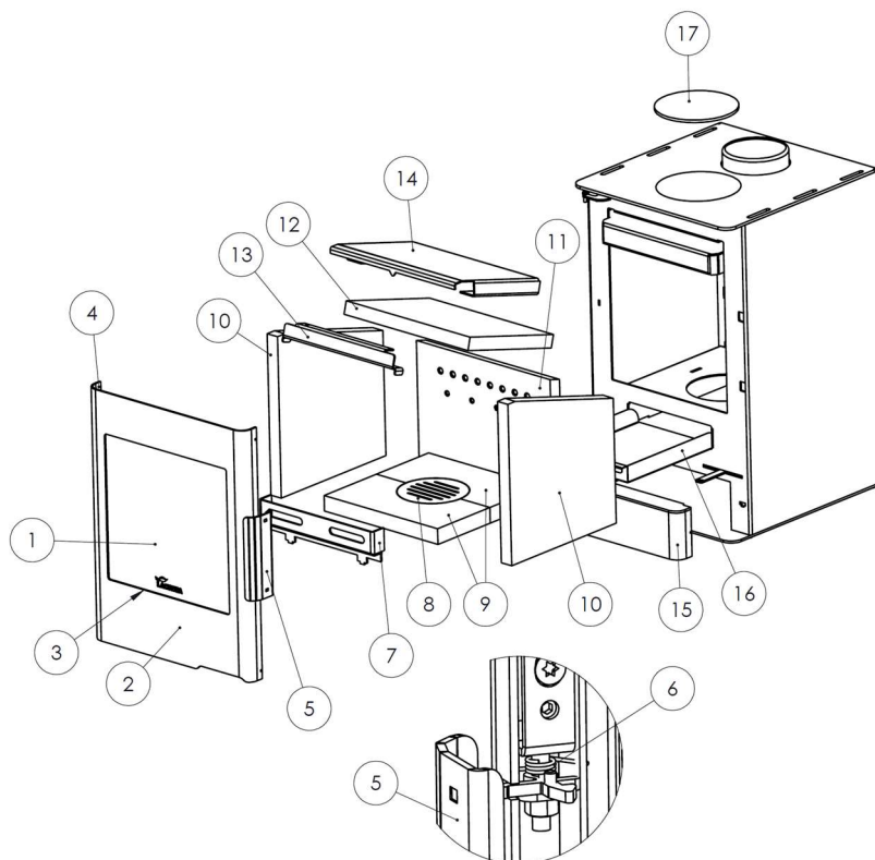
Figure nº7 - Despiece NOMAD
