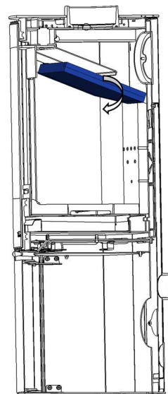
Figure n°17 - Retirer la vermiculite
