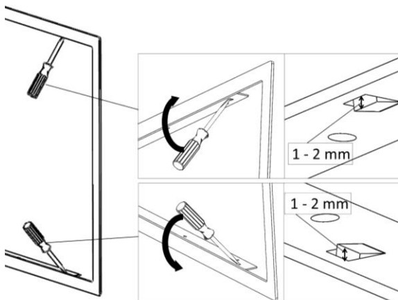
Figure n°11 - Tirer les Clips
