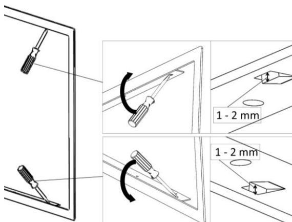
Figure n°13 - Tirer les Clips
