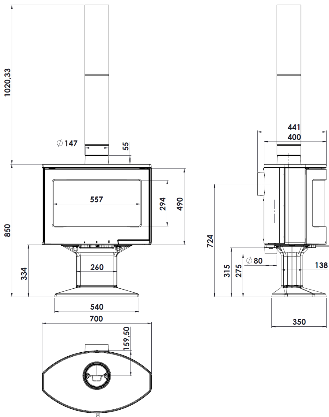
Figure No.1 - Dimensions of the Tarbes Star appliance in mm
