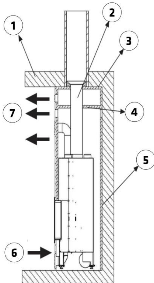
Figure No.5 - Interior diagram of the casing
