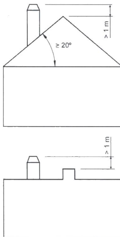
Figure No.7 - Distances between chimney crown and roof ridge
