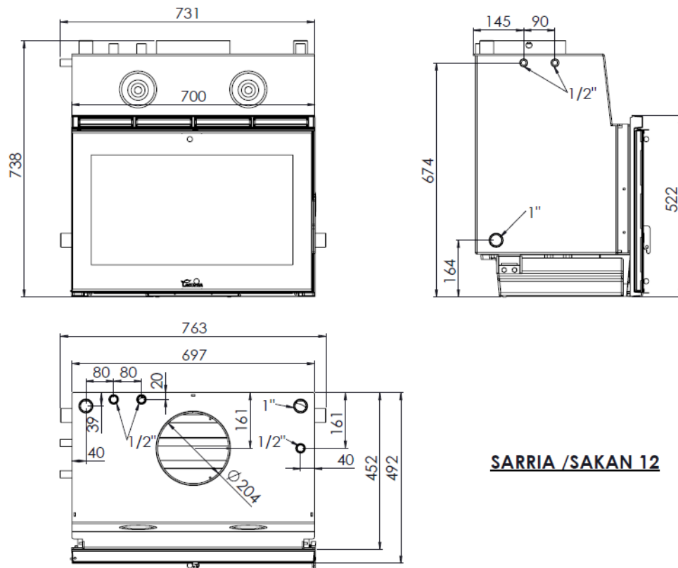
Figure No.1 - Dimensions of the SARRIA SAKAN 12 appliance in mm
