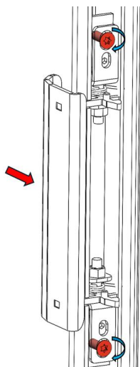
Figure No.19 - STEP 3: Tighten screws to reattach the system
