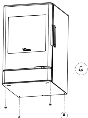
Figure No.16 - Installation of leveling feet
