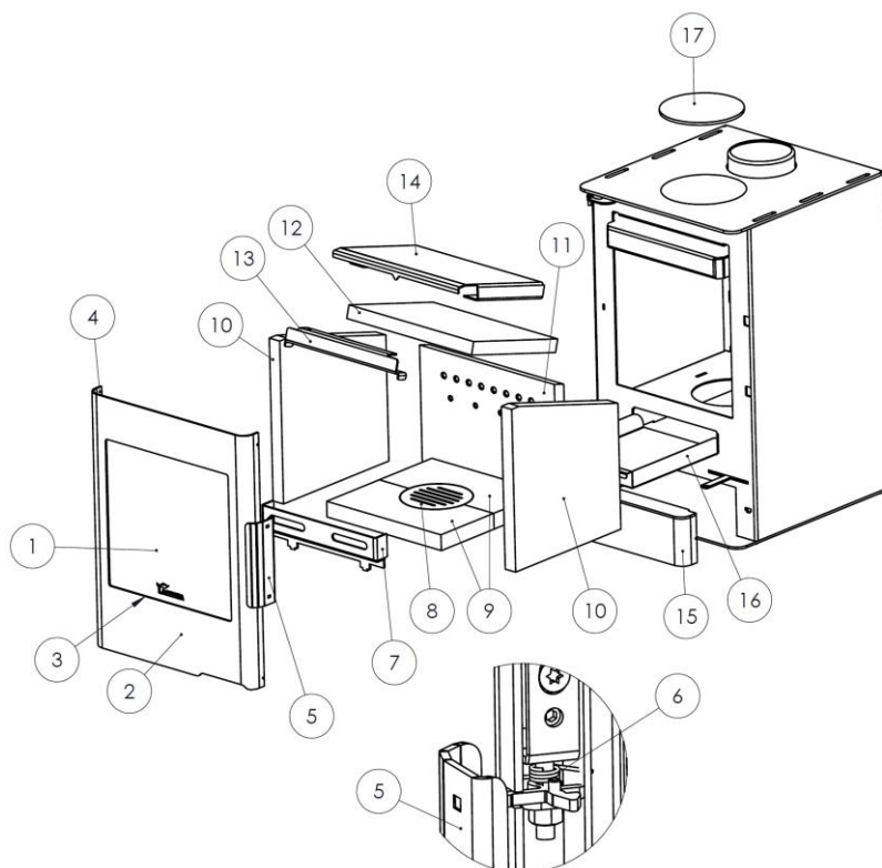
Figure No.23 - NOMAD Exploded View
