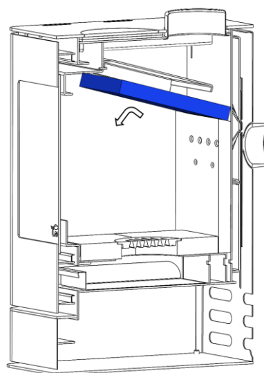
Figure No.14 - Remove the vermiculite deflector
