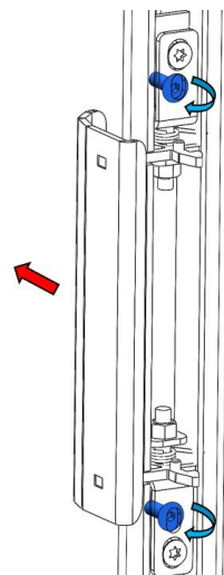
Figure No.21 - STEP 2: Tighten the screws that regulate the depth to where we are interested
