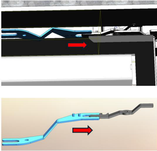
Figure No.39 - Insert the tool into the upper right rotating lever
