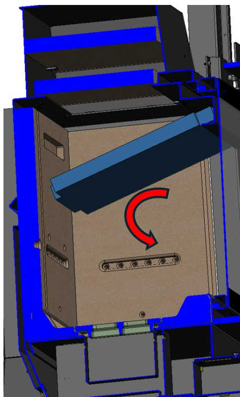
Figure No.35 - Removing the lower Izaro 100 CLI deflector
