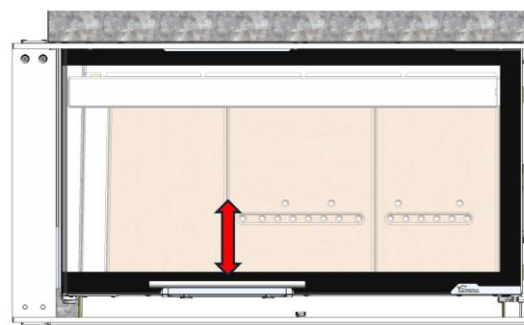
Figure No.38 - Opening using guillotine system
