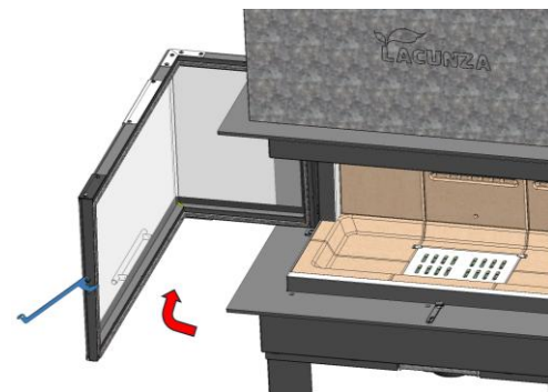
Figure No.43 - Door open horizontally
