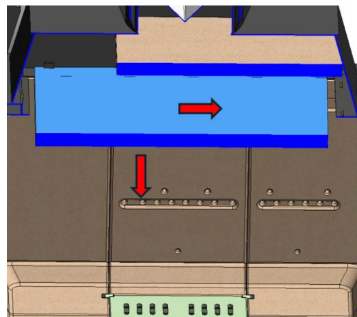
Figure No.36 - Removing the middle deflector on the Izaro 100 CLI
