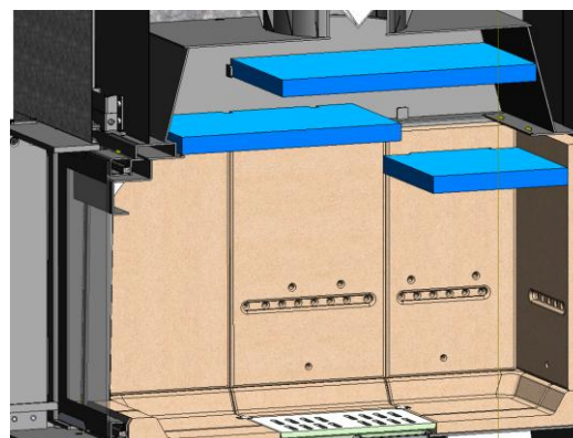
Figure No.34 - Section view with Izaro 100 CLI deflectors fitted.
