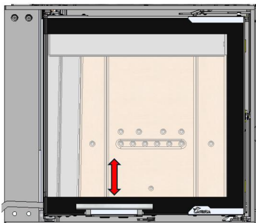
Figure No.36 - Opening using guillotine system
