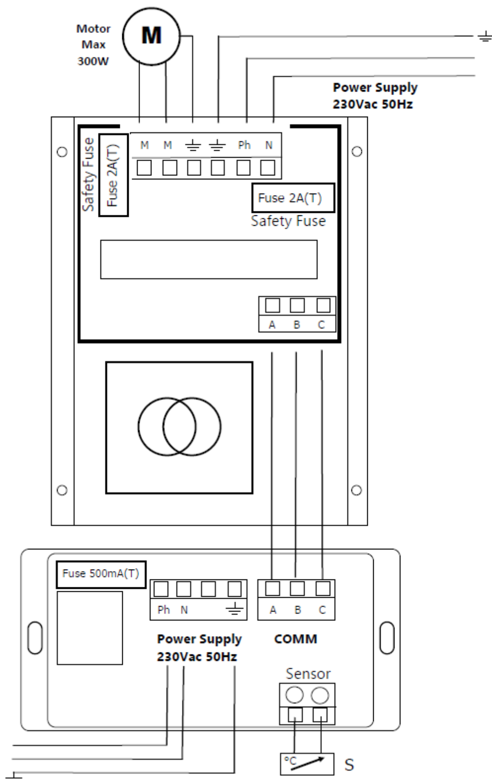
Figure No.18 - Connections to be made in the controller and the power module of the Izaro C/V
