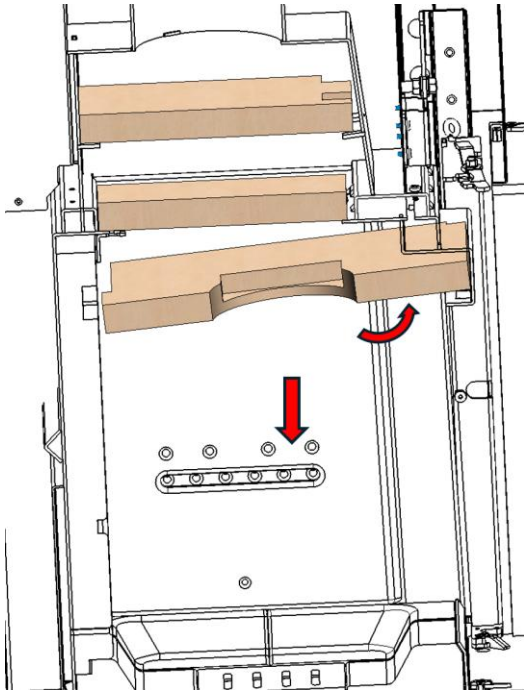
Figure No.32 - Removing the lower right deflector (side opposite the side glass)
