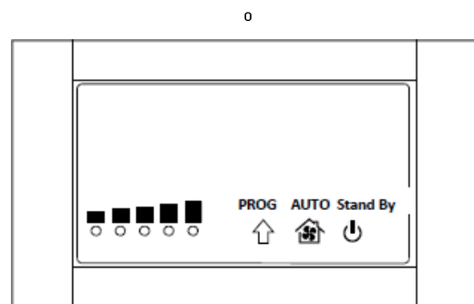
Figure No.43 - Izaro air regulator automatic/progressive display
