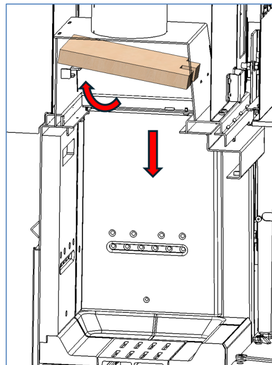
Figure No.35 - Removing the Izaro 60 CLI upper deflector
