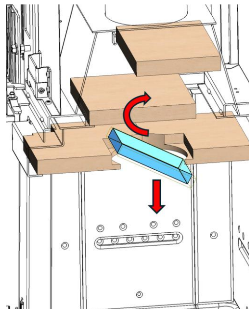
Figure No.31 - Removing the Izaro 60 CLI catalyst
