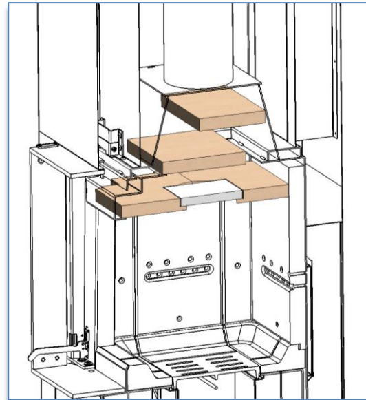
Figure No.30 - Section view with Izaro 60 CLI 3 deflectors fitted.
