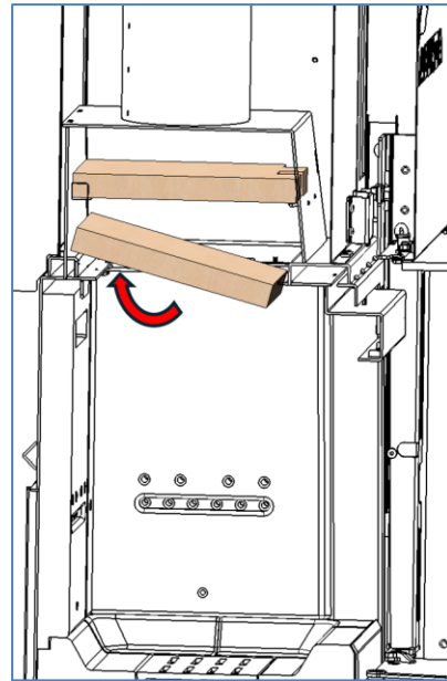
Figure No.34 - Removing the Izaro 60 CLI middle deflector
