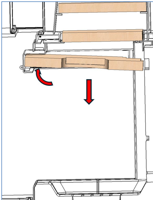
Figure No.33 - Removing the lower deflector Left (side glass side)
