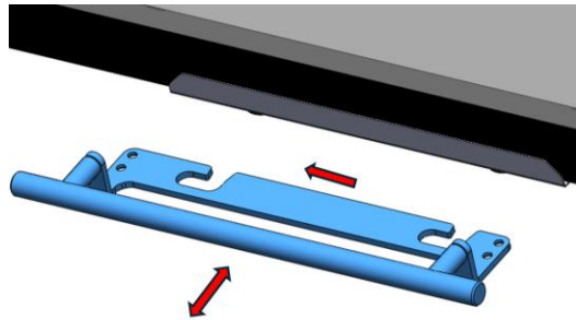
Figure No.42 - Screw removal and use as a cold handle handle
