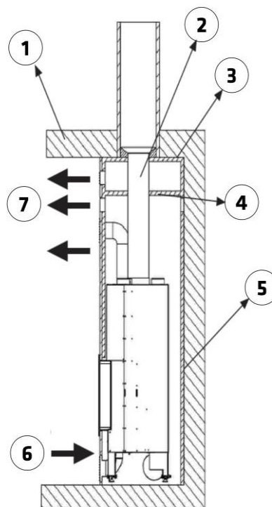
Figure No.6 - Interior diagram of the casing
