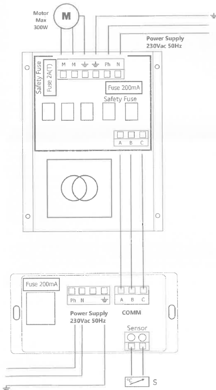
Figure No.17 - Connections to be made in the controller and the power module of the Itaca eco
