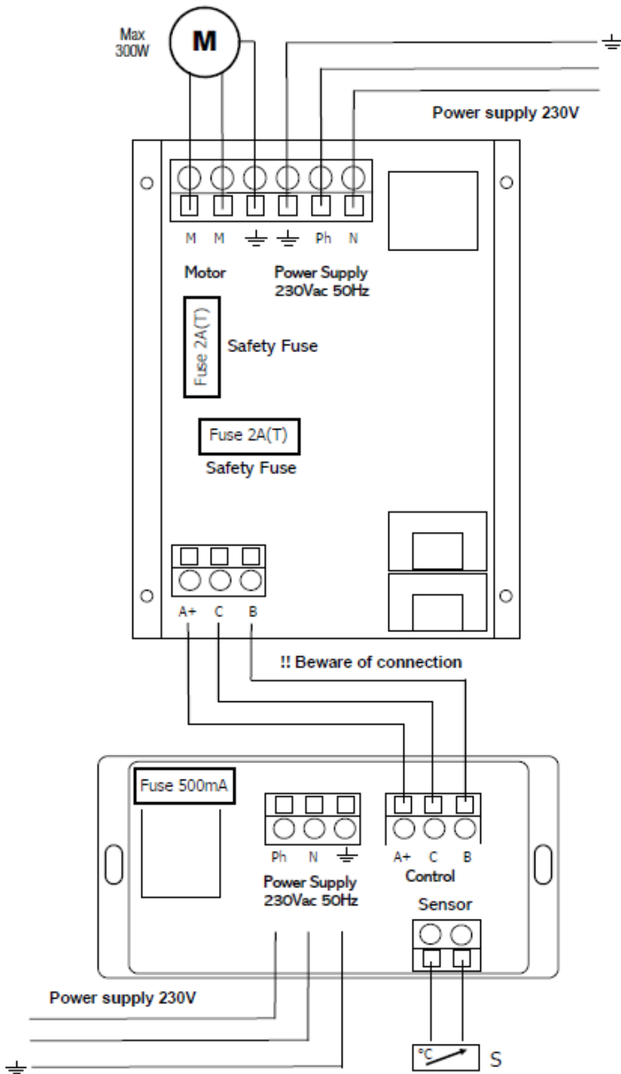
Figure No.17 - Connections to be made in the controller and the power module of the Itaca eco
