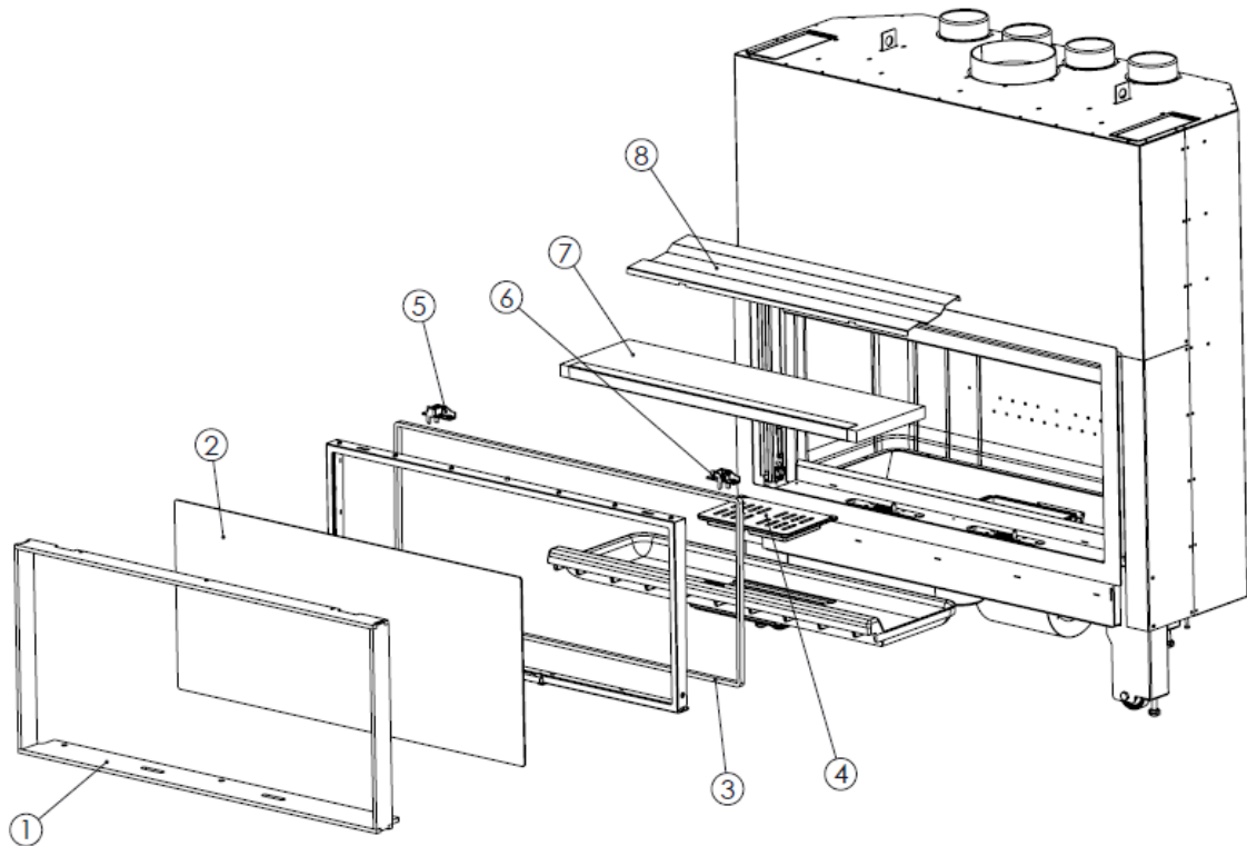
Figure No.51 - Itaca 100-120 eco Basic breakdowns
