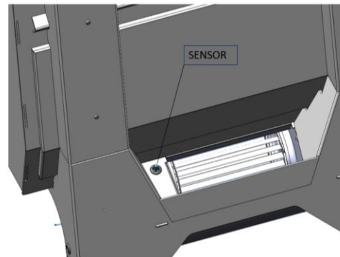
Figure No.21 - Position of the temperature probe (SENSOR) in the turbine air outlet
