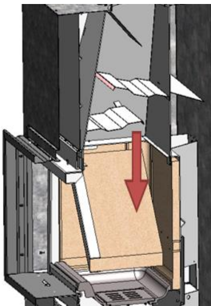
Figure No.31 - Dismantling the lower Itaca 80 eco deflector
