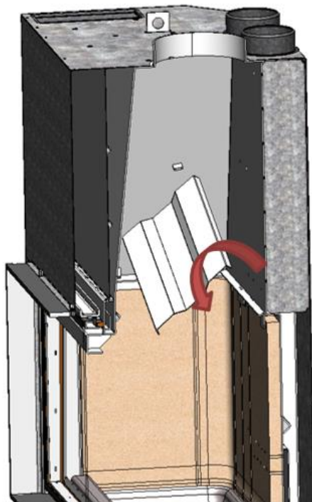
Figure No.35 - Removing the second deflector on the Itaca 100-120 eco
