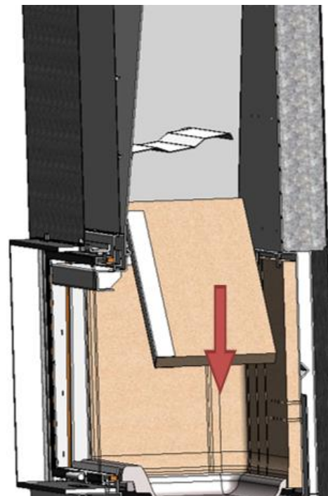
Figure No.34 - Dismantling the lower Itaca 100 y 120 eco deflector
