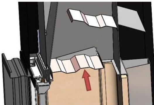
Figure No.21 - Removing the middle deflector on the Inca
