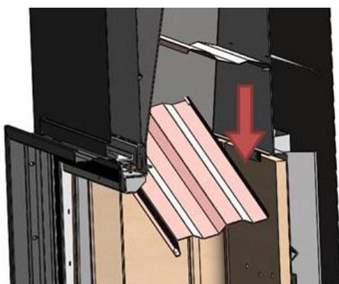
Figure No.20 - Dismantling the lower Inca deflector
