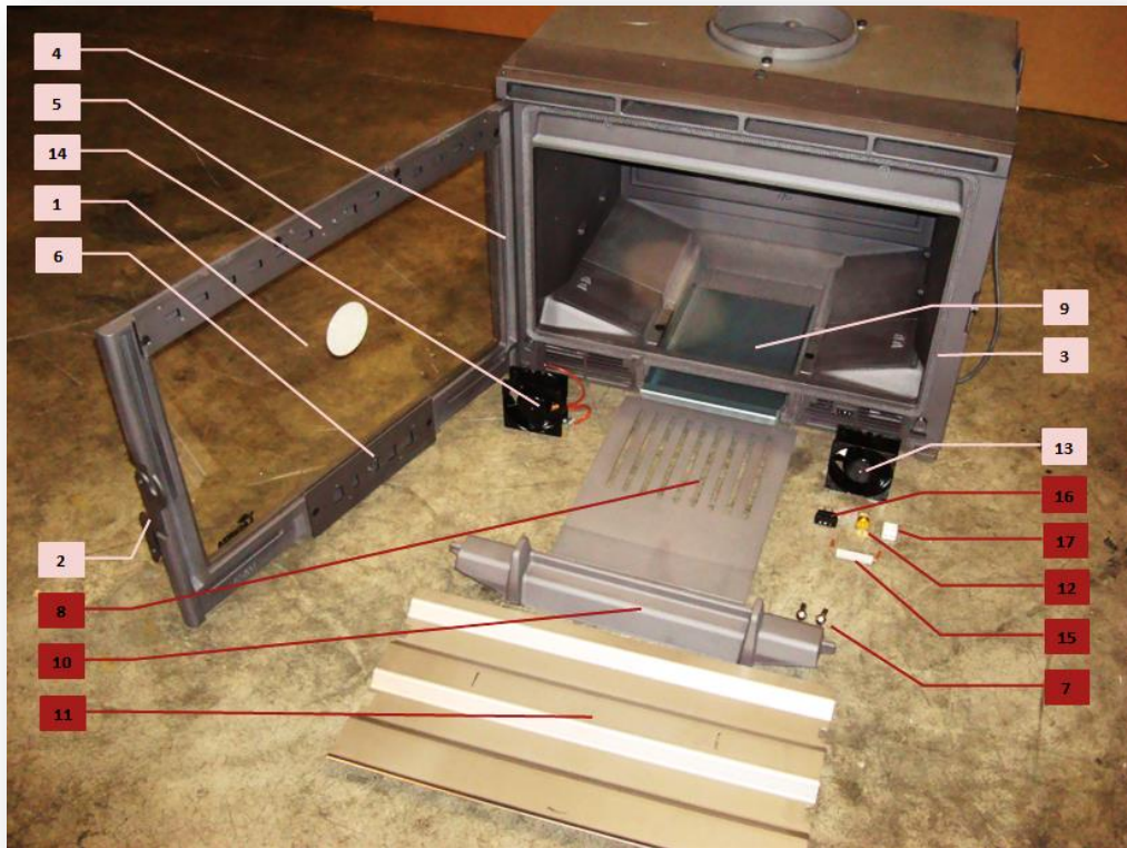
Figure No.12 - Basic breakdowns
