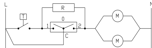
Figure No.11 - Electrical diagram for fans
