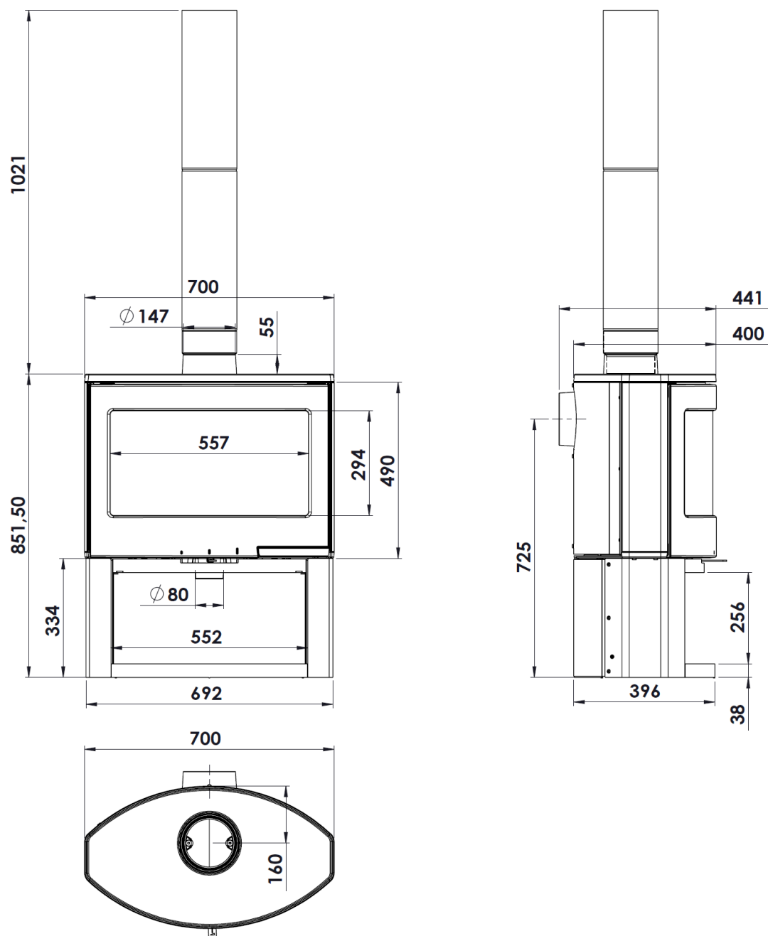
Figure No.1 - Dimensions of the Dublin Star / Bristol Star appliance in mm
