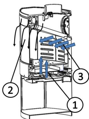
Figure No.19 - Combustion air intakes
