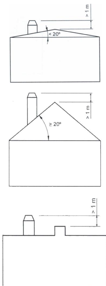
Figure No.14 - Distances between chimney crown and roof ridge
