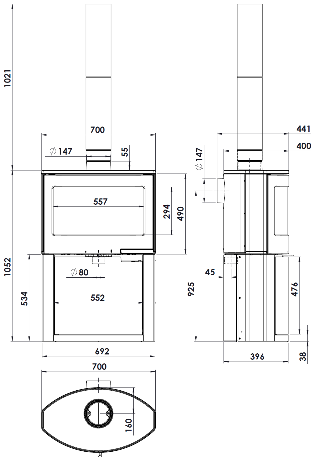
Figure No.2 - Dimensions of the Bera Star appliance
