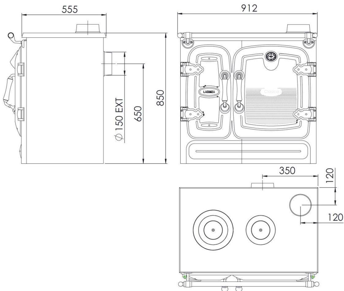
Figure No.2 - Dimensions of the Clásica 7T appliance in mm
