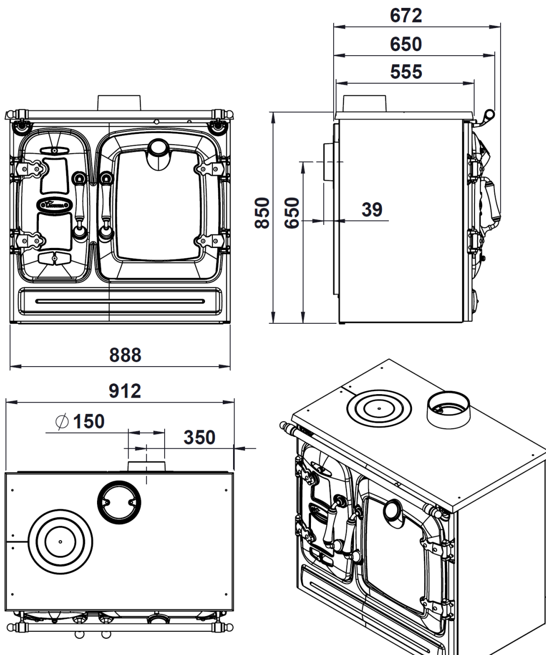
Figure No.2 - Dimensions of the Clásica 7T appliance in mm
