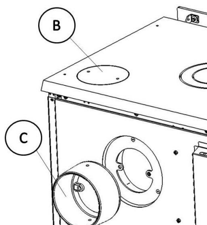
Figure No.8 - Diagram for rear flue socket
