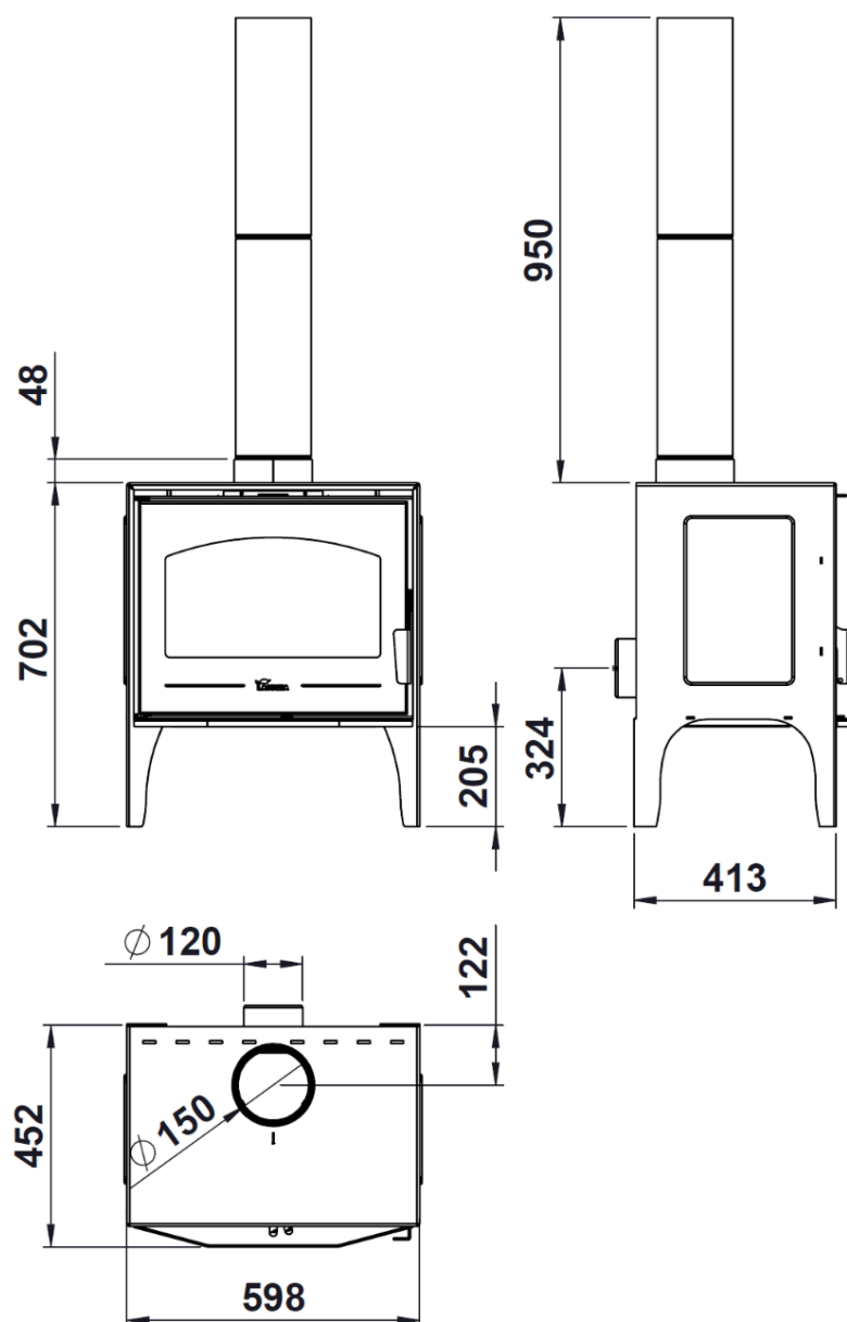
Figure No.1 - Dimensions of the CALPE STAR series in mm
