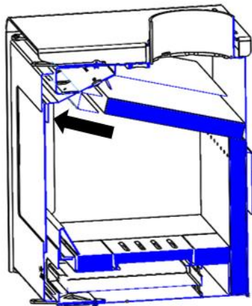
Figure No.9 - First movement to release the reinforcement
