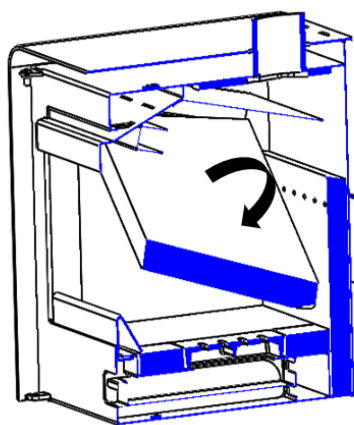
Figure No.10 - Extracting the vermiculite deflectors
