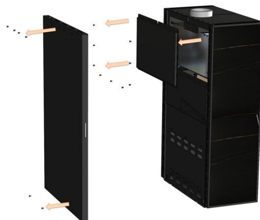
Figure No.19 - Remove the back cover Bergen
