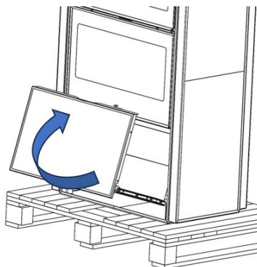
Figure No.4 - Detail of drawer removal
