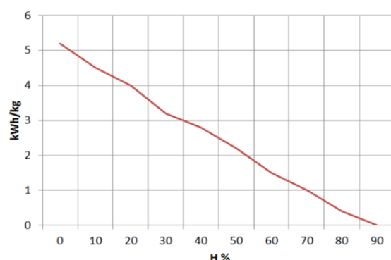
Figure No.23 - Relationship between firewood humidity and heat output
