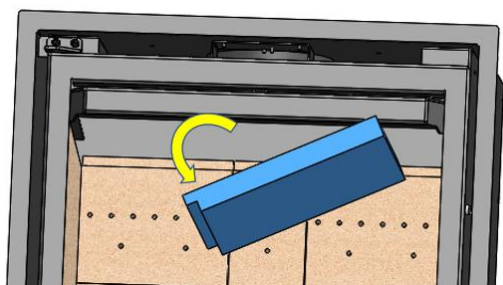
Figure No.26 - Dismantling the vermiculite deflector
