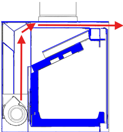
Figure No.16 - Hot air flow without ducting
