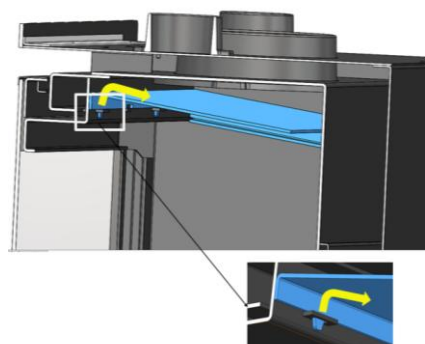
Figure No.27 - Dismantling the steel deflector
