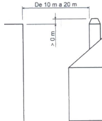
Figure No.21 - Distances between the chimney crown and objects within a radius of between 10 and 20m
