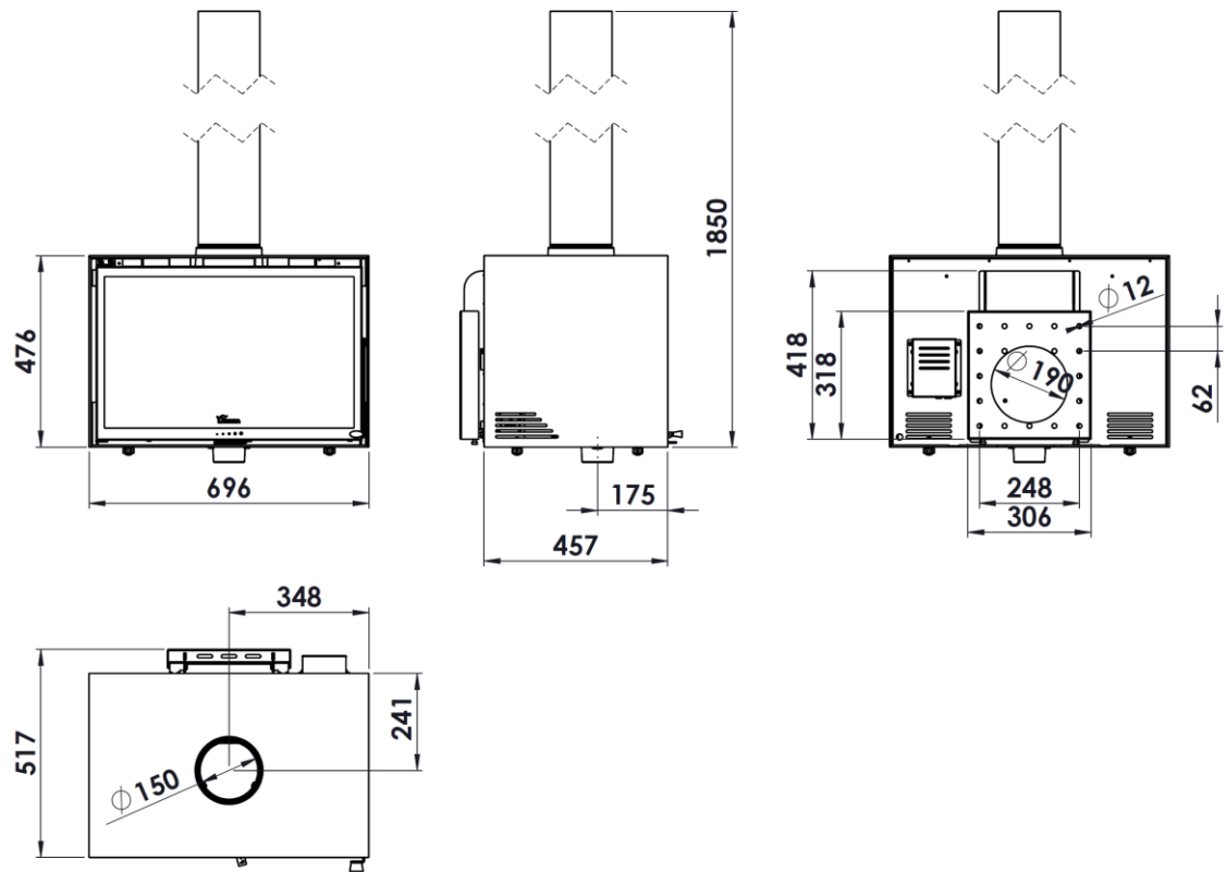
Figure No.2 - Dimensions of the BAIONA 700 STAR MURAL appliance in mm
