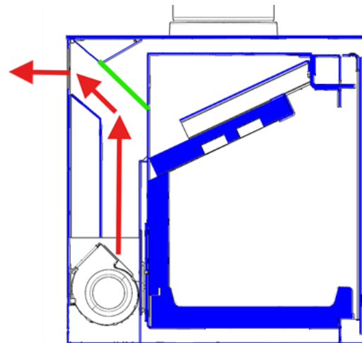
Figure No.18 - Hot air flow with ducting
