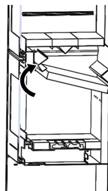
Figure No.15 - Stainless-steel reinforcement in its closed position
