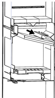
Figure No.13 - Reinforcement on the vermiculite deflectors
