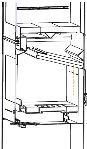
Figure No.17 - Stainless-steel reinforcement in its open position
