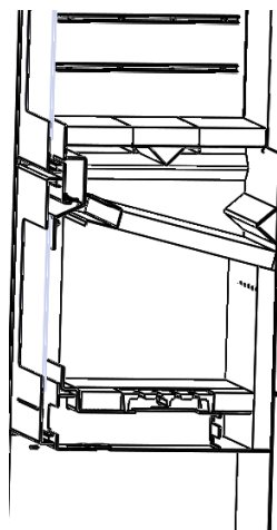
Figure No.15 - Stainless-steel reinforcement in its closed position
