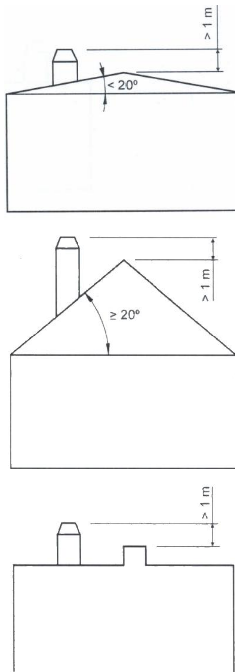
Figure No.3 - Distances between chimney crown and roof ridge
