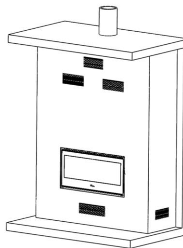
Figure No.6 - Exterior diagram of the casing
